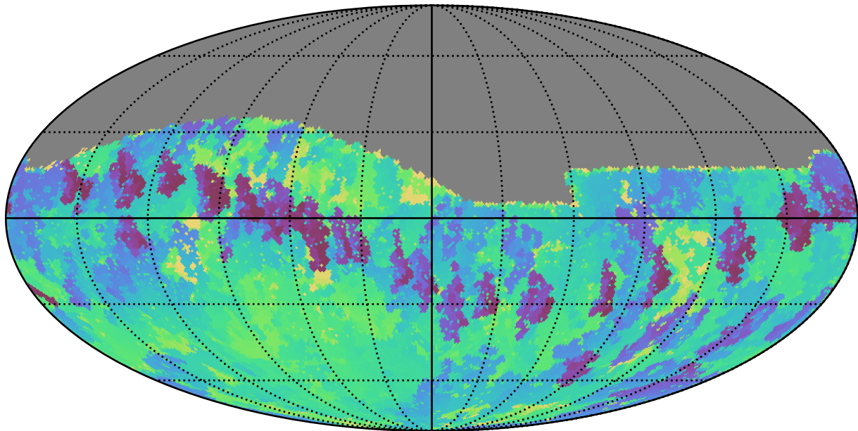
ddf_loaded_half_fl1_v3.4_10yrs Yr 1 i band: Min skyBrightness
