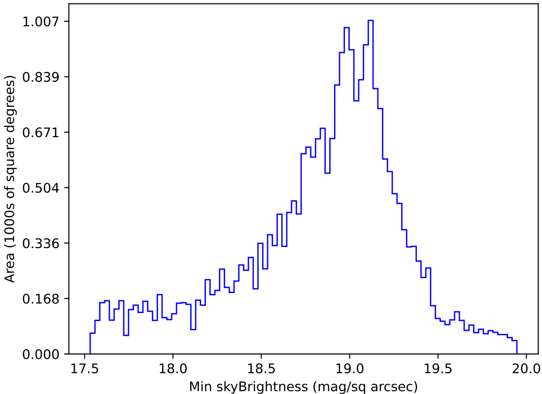
ddf_loaded_half_fl1_v3.4_10yrs Yr 1 i band: Min skyBrightness
