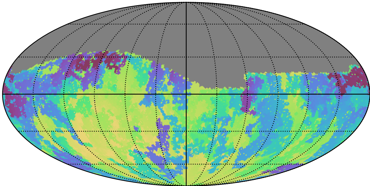
ddf_loaded_half_fl1_v3.4_10yrs Yr 1 g band: Min skyBrightness
