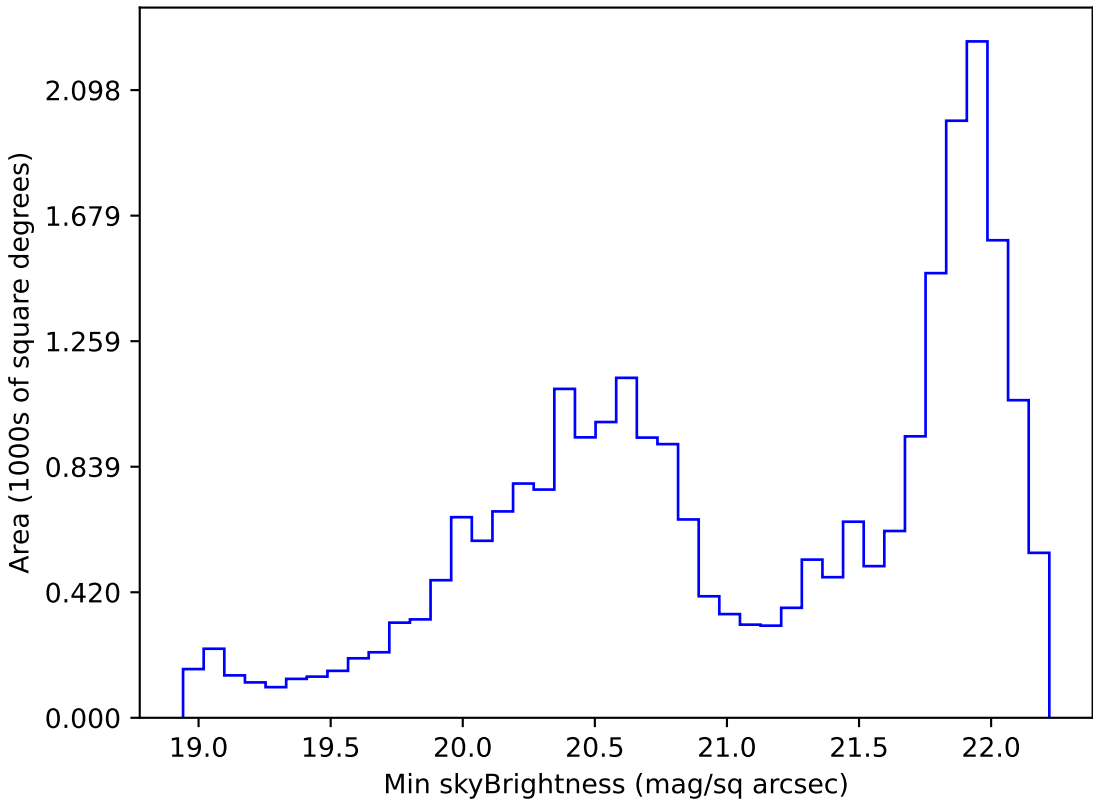
ddf_loaded_half_fl1_v3.4_10yrs Yr 1 g band: Min skyBrightness
