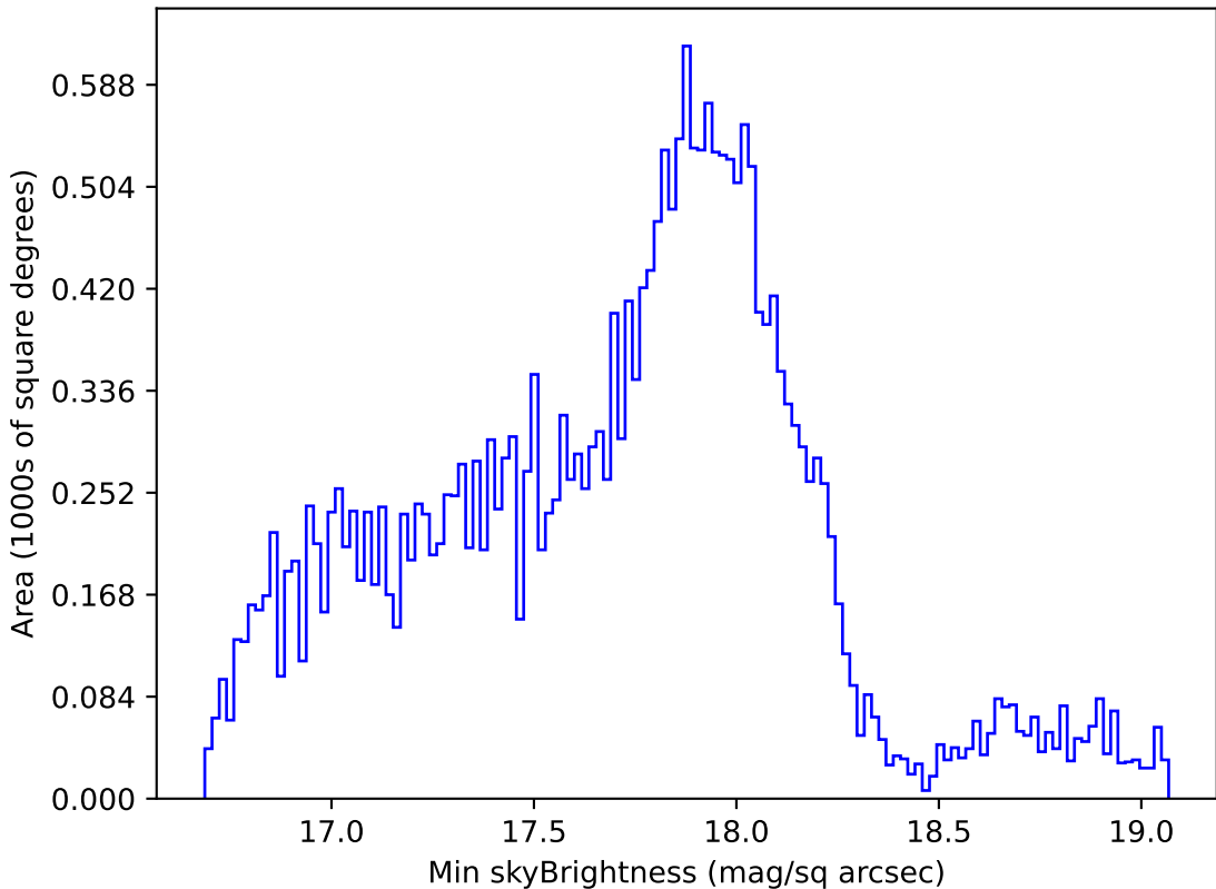
ddf_loaded_half_fl1_v3.4_10yrs Yr 1 all bands: Min skyBrightness
