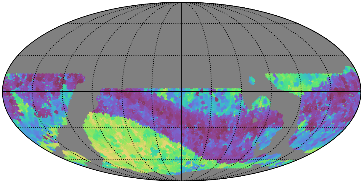
ddf_loaded_half_fl1_v3.4_10yrs WFD z band: Min skyBrightness
