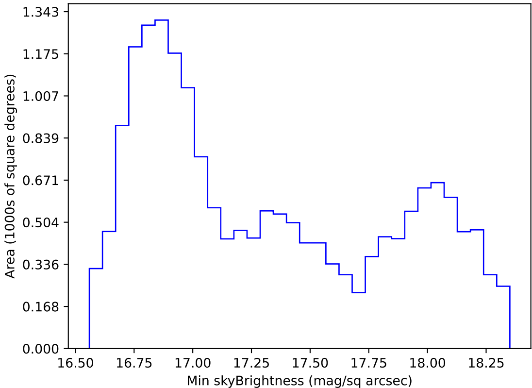
ddf_loaded_half_fl1_v3.4_10yrs WFD z band: Min skyBrightness
