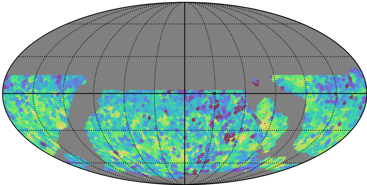
ddf_loaded_half_fl1_v3.4_10yrs WFD y band: Min skyBrightness
