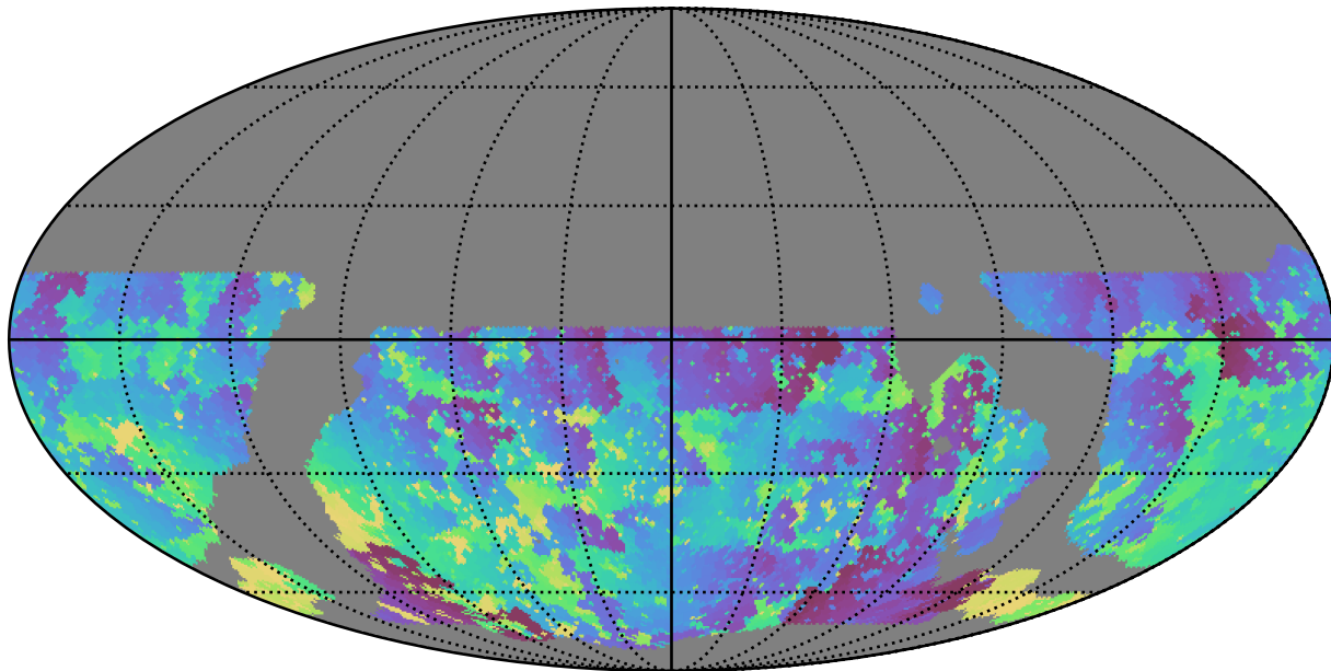
ddf_loaded_half_fl1_v3.4_10yrs WFD u band: Min skyBrightness
