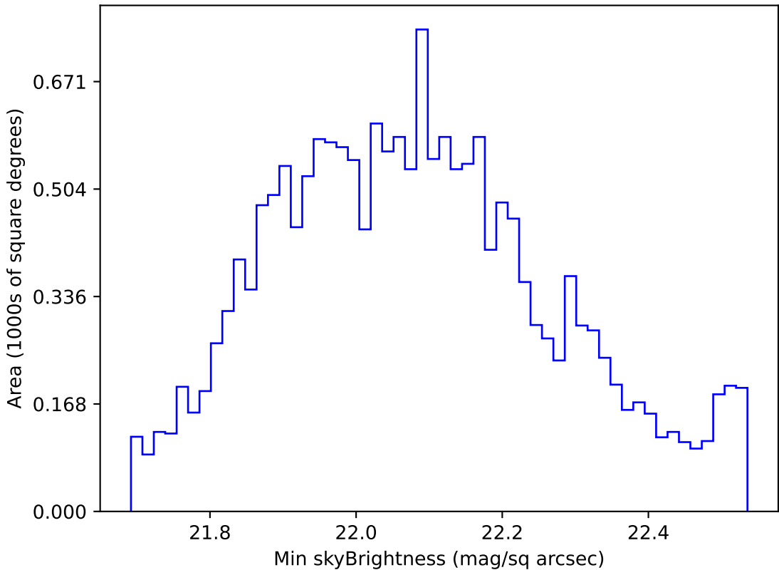
ddf_loaded_half_fl1_v3.4_10yrs WFD u band: Min skyBrightness
