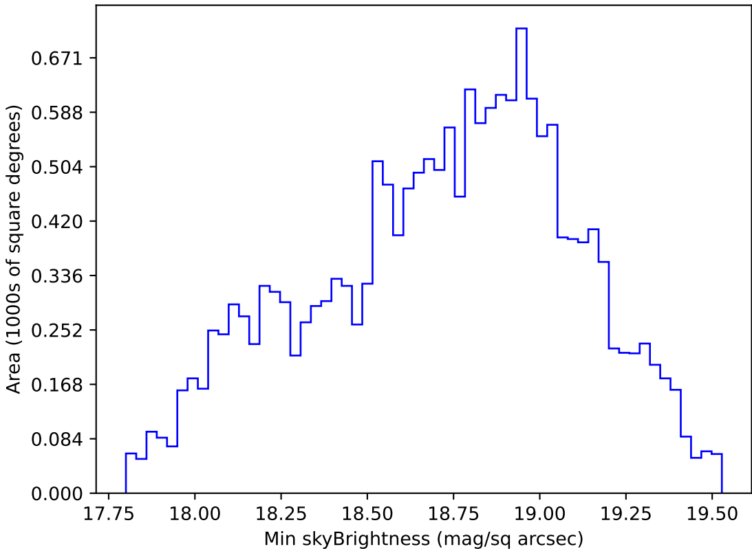
ddf_loaded_half_fl1_v3.4_10yrs WFD r band: Min skyBrightness
