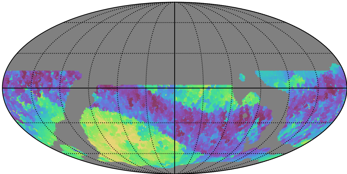
ddf_loaded_half_fl1_v3.4_10yrs WFD i band: Min skyBrightness
