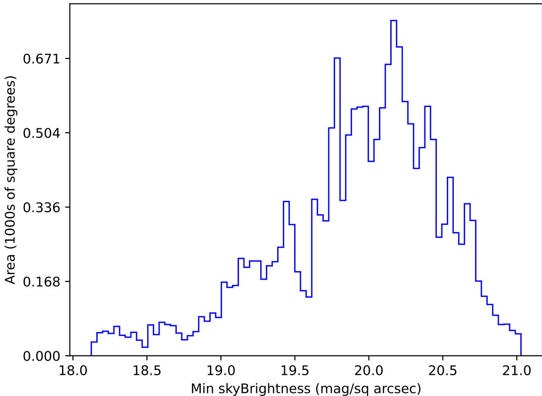
ddf_loaded_half_fl1_v3.4_10yrs WFD g band: Min skyBrightness
