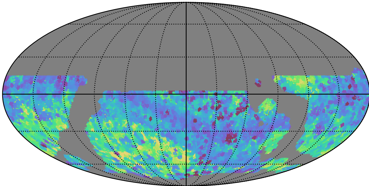
ddf_loaded_half_fl1_v3.4_10yrs WFD all bands: Min skyBrightness
