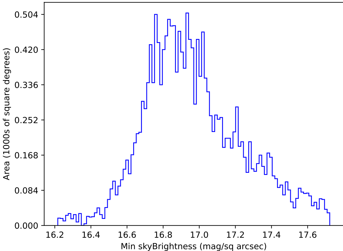
ddf_loaded_half_fl1_v3.4_10yrs WFD all bands: Min skyBrightness
