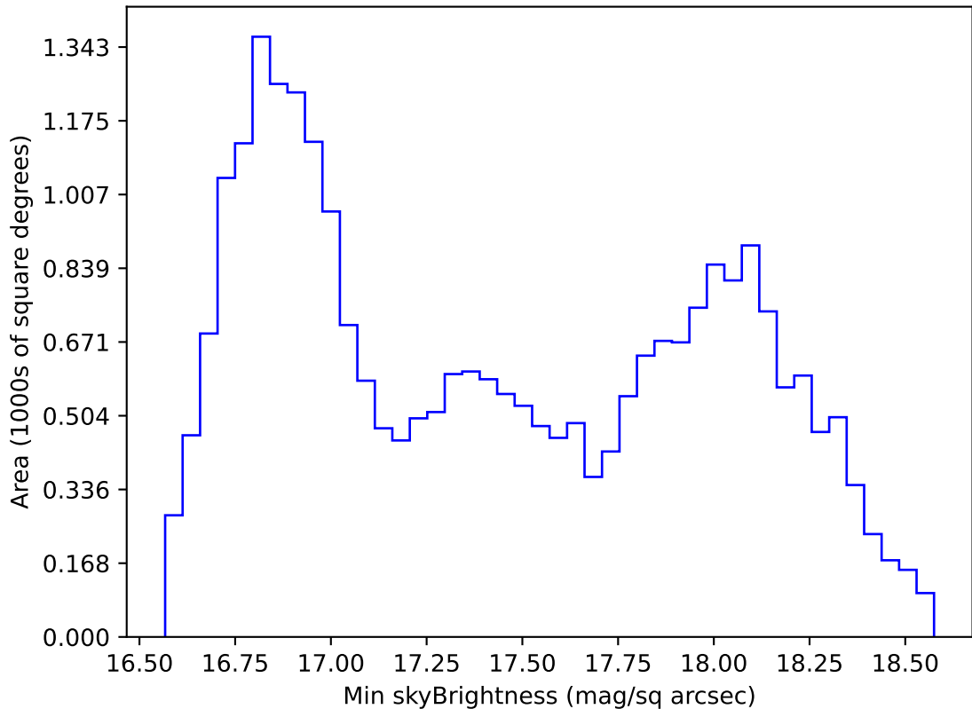
ddf_loaded_half_fl1_v3.4_10yrs All sky z band: Min skyBrightness
