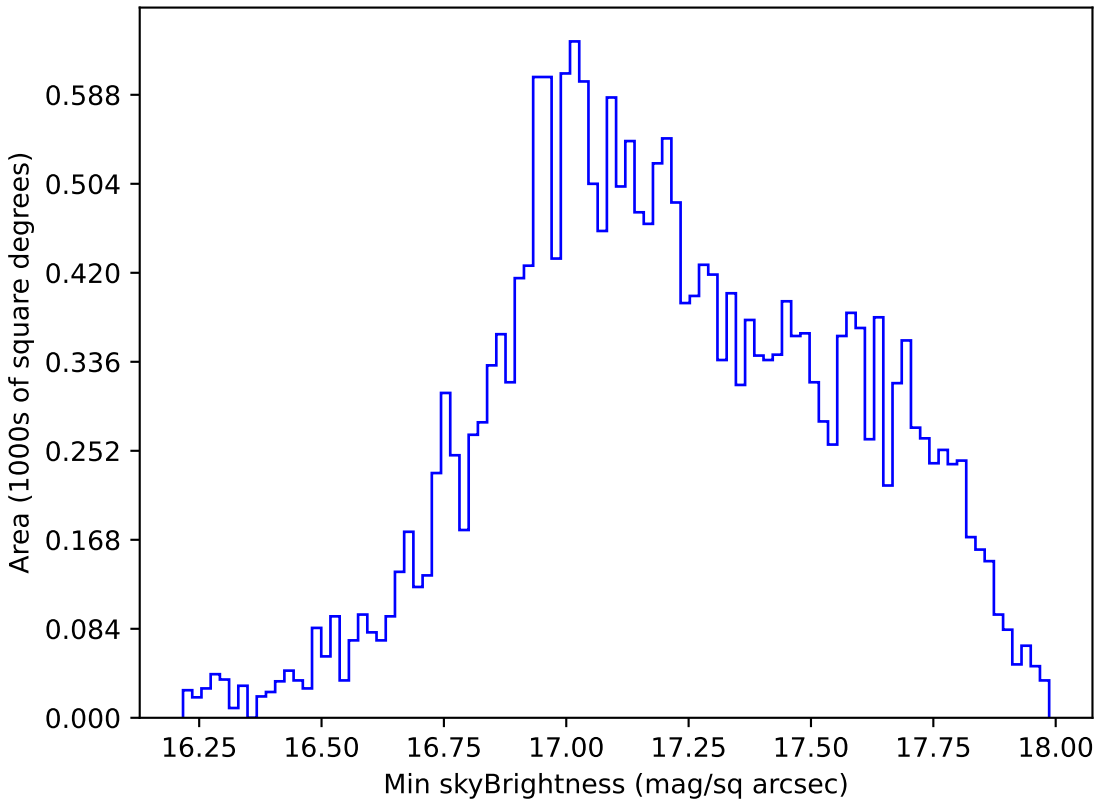
ddf_loaded_half_fl1_v3.4_10yrs All sky y band: Min skyBrightness
