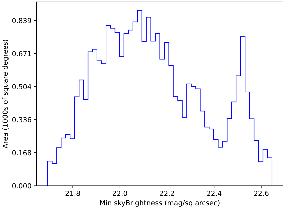
ddf_loaded_half_fl1_v3.4_10yrs All sky u band: Min skyBrightness
