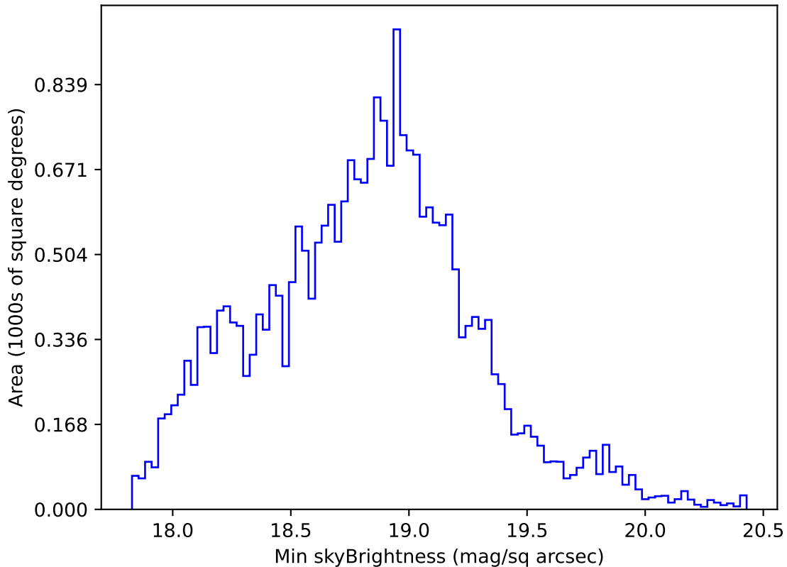
ddf_loaded_half_fl1_v3.4_10yrs All sky r band: Min skyBrightness
