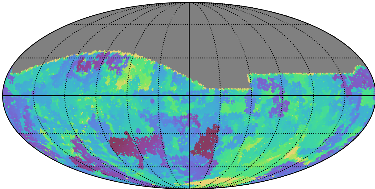
ddf_loaded_half_fl1_v3.4_10yrs All sky g band: Min skyBrightness
