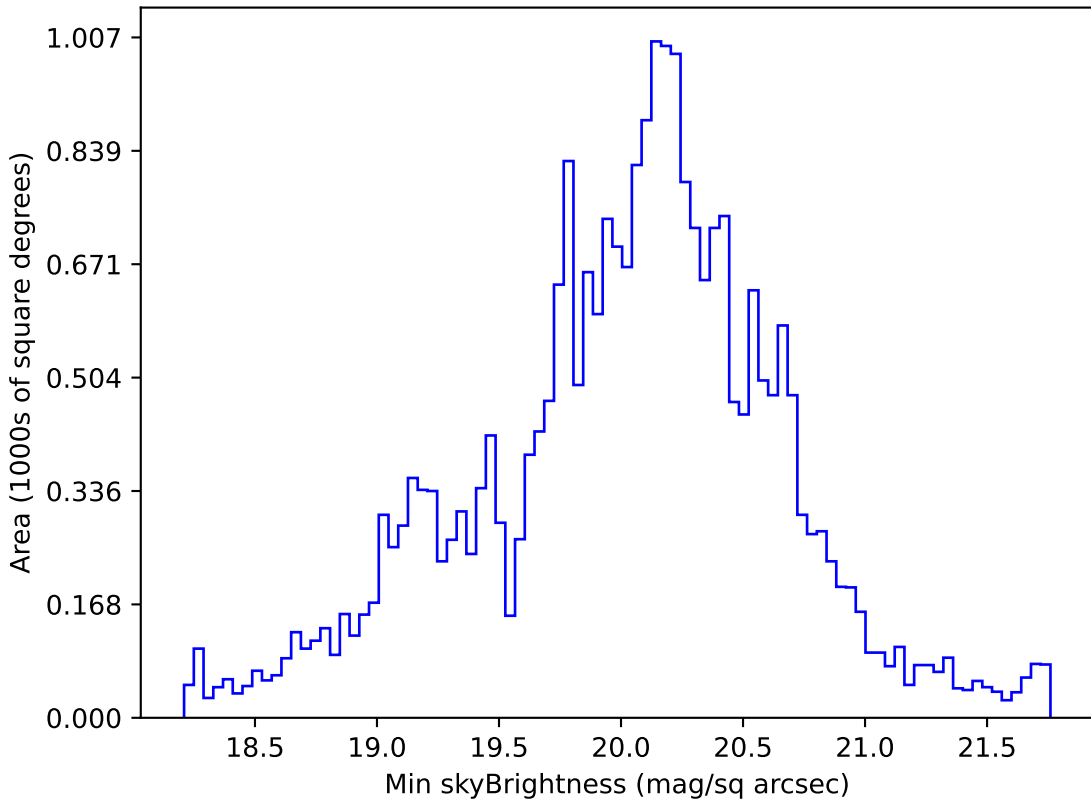
ddf_loaded_half_fl1_v3.4_10yrs All sky g band: Min skyBrightness
