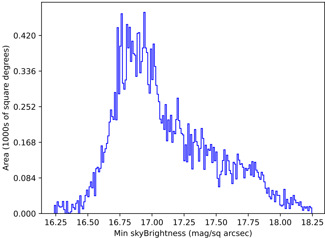
ddf_loaded_half_fl1_v3.4_10yrs All sky all bands: Min skyBrightness
