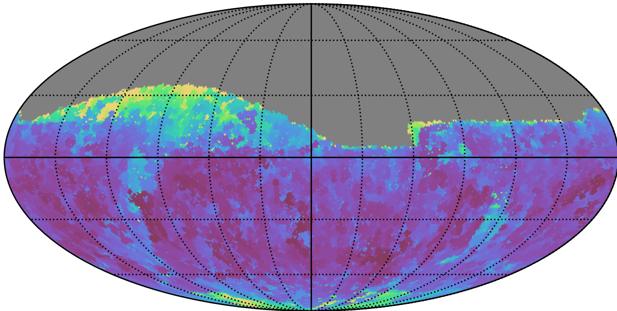
ddf_loaded_half_fl1_v3.4_10yrs Yr 1 z band: Min seeingGeom
