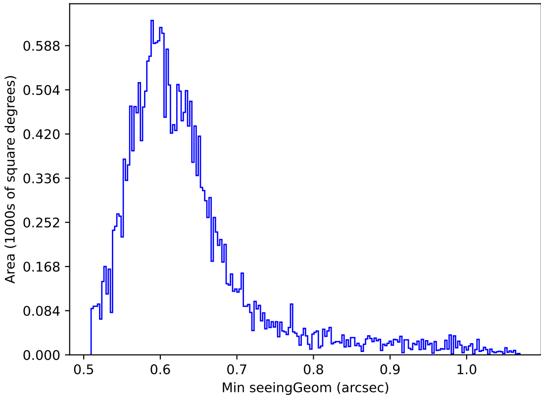
ddf_loaded_half_fl1_v3.4_10yrs Yr 1 r band: Min seeingGeom
