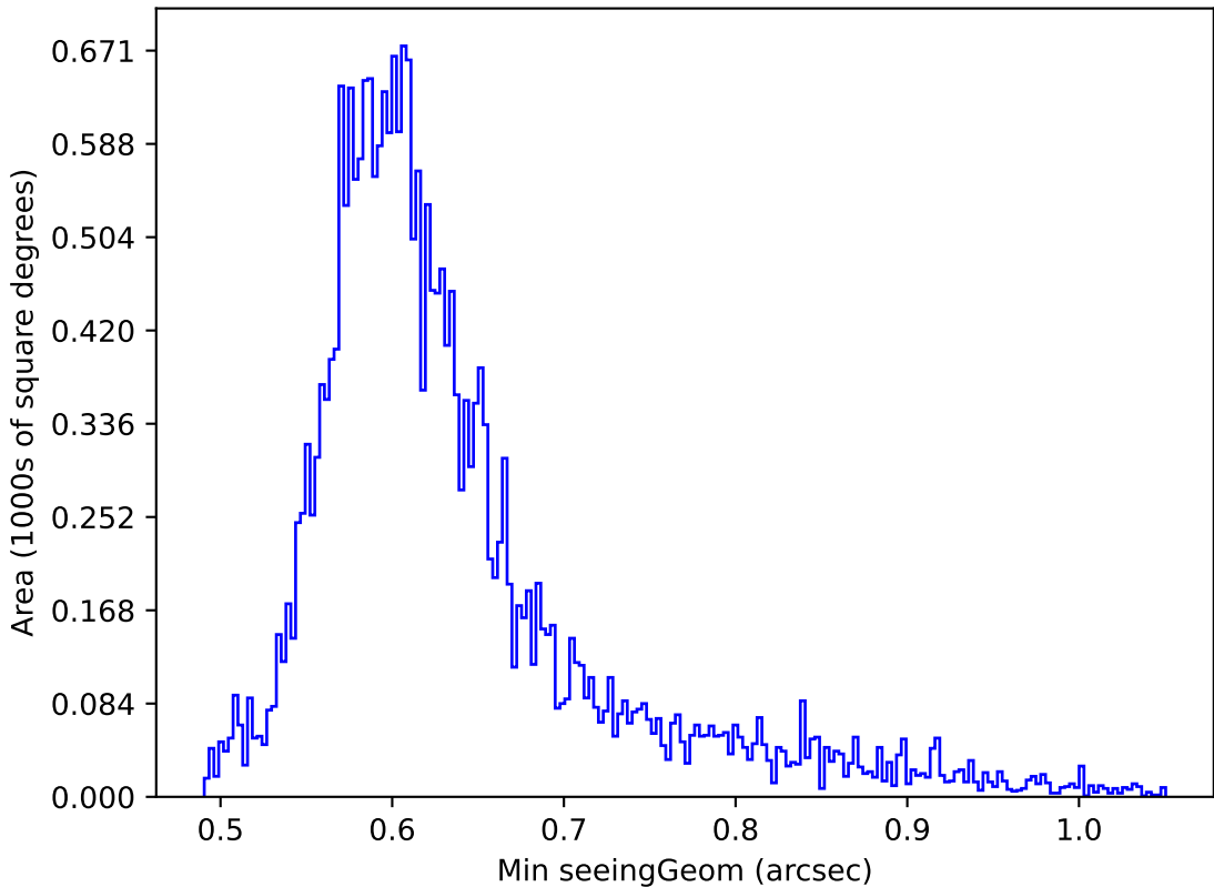
ddf_loaded_half_fl1_v3.4_10yrs Yr 1 i band: Min seeingGeom
