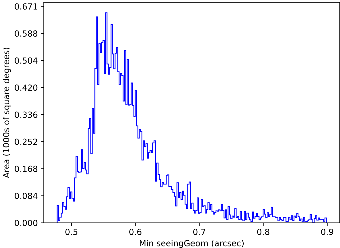
ddf_loaded_half_fl1_v3.4_10yrs Yr 1 all bands: Min seeingGeom
