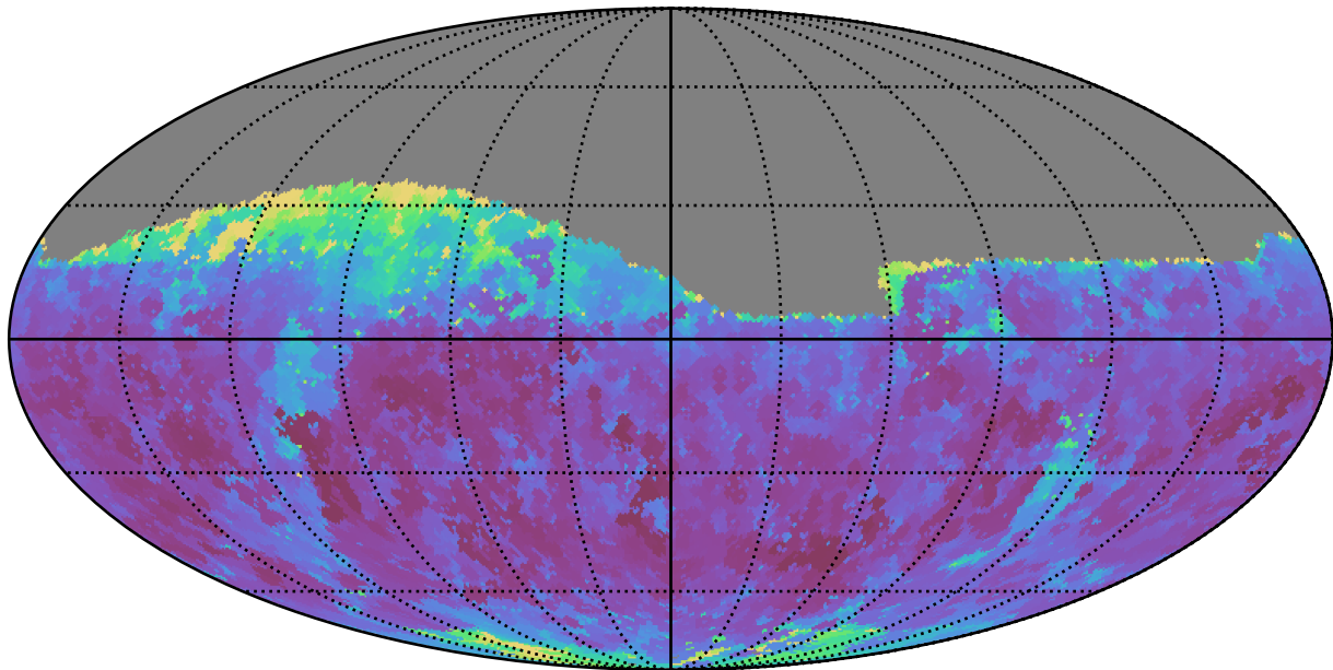
ddf_loaded_half_fl1_v3.4_10yrs Yr 1 z band: Min seeingEff
