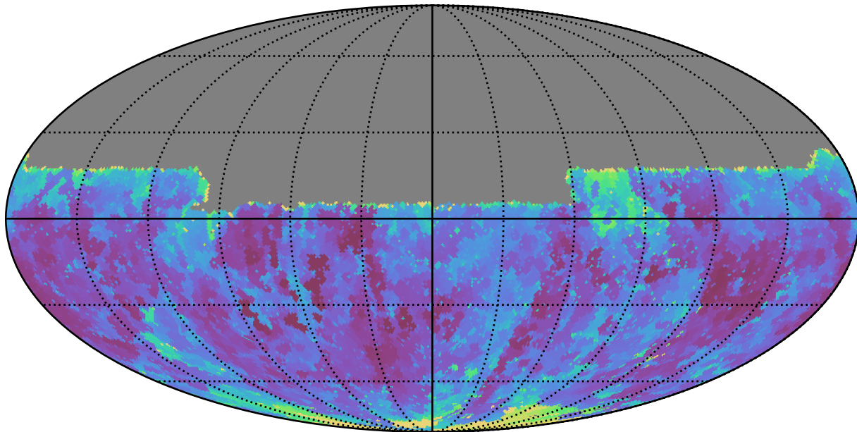
ddf_loaded_half_fl1_v3.4_10yrs Yr 1 y band: Min seeingEff
