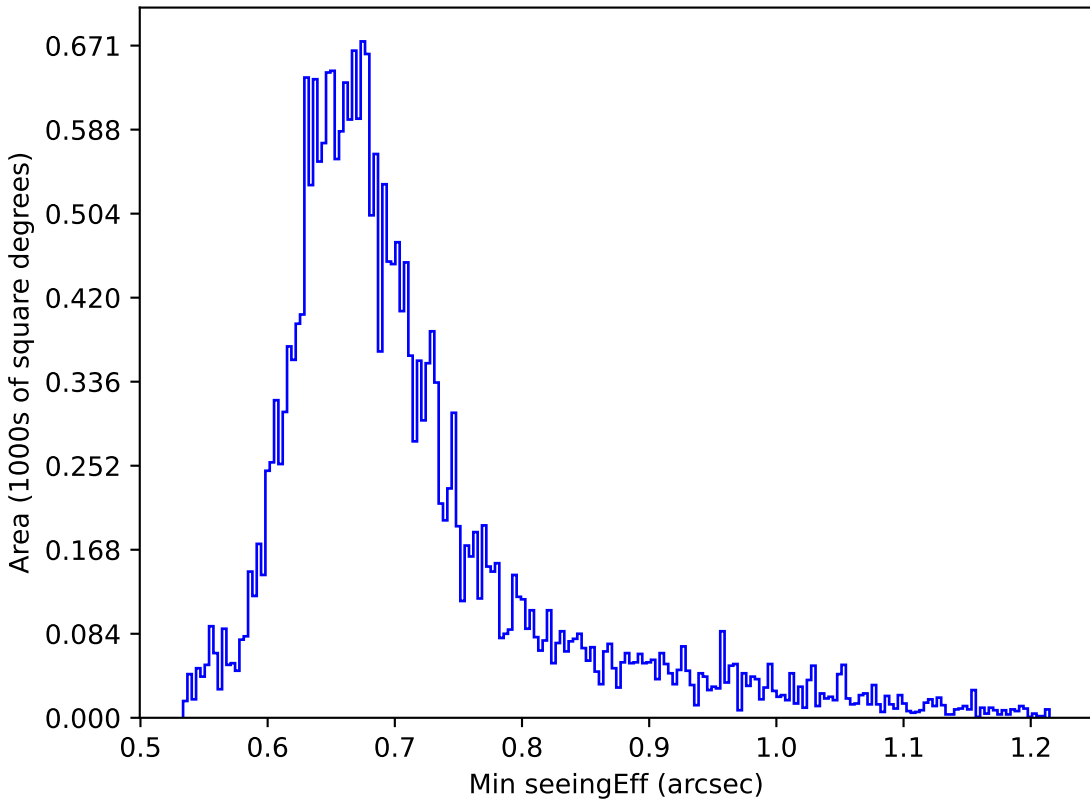
ddf_loaded_half_fl1_v3.4_10yrs Yr 1 i band: Min seeingEff
