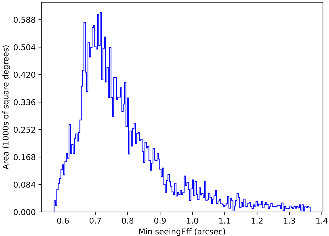
ddf_loaded_half_fl1_v3.4_10yrs Yr 1 g band: Min seeingEff
