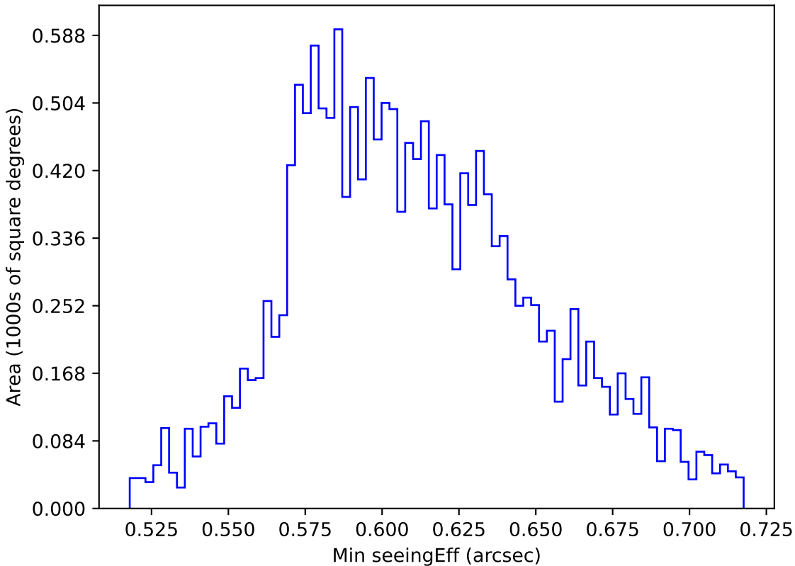
ddf_loaded_half_fl1_v3.4_10yrs WFD z band: Min seeingEff
