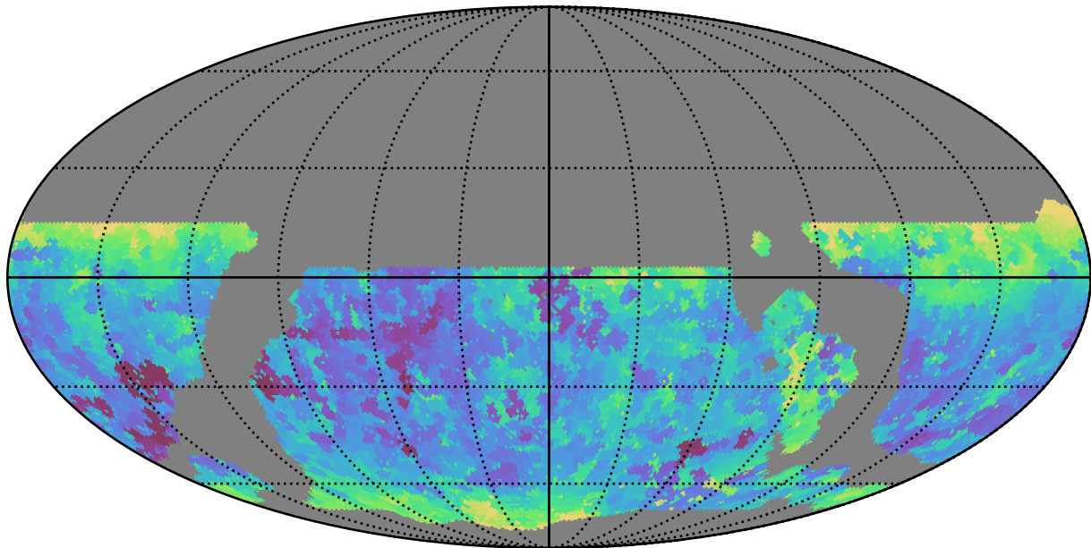
ddf_loaded_half_fl1_v3.4_10yrs WFD y band: Min seeingEff
