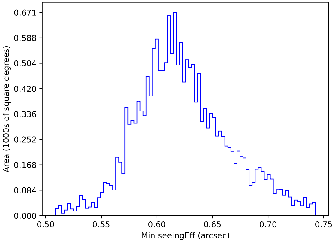
ddf_loaded_half_fl1_v3.4_10yrs WFD y band: Min seeingEff
