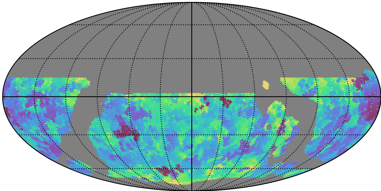
ddf_loaded_half_fl1_v3.4_10yrs WFD u band: Min seeingEff
