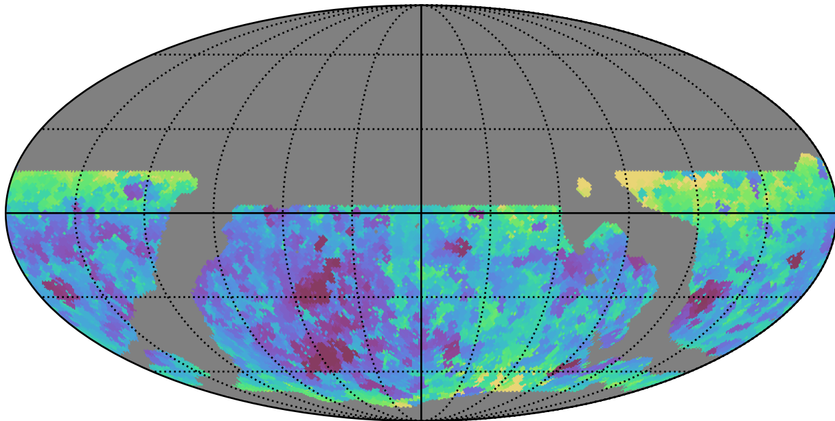
ddf_loaded_half_fl1_v3.4_10yrs WFD r band: Min seeingEff
