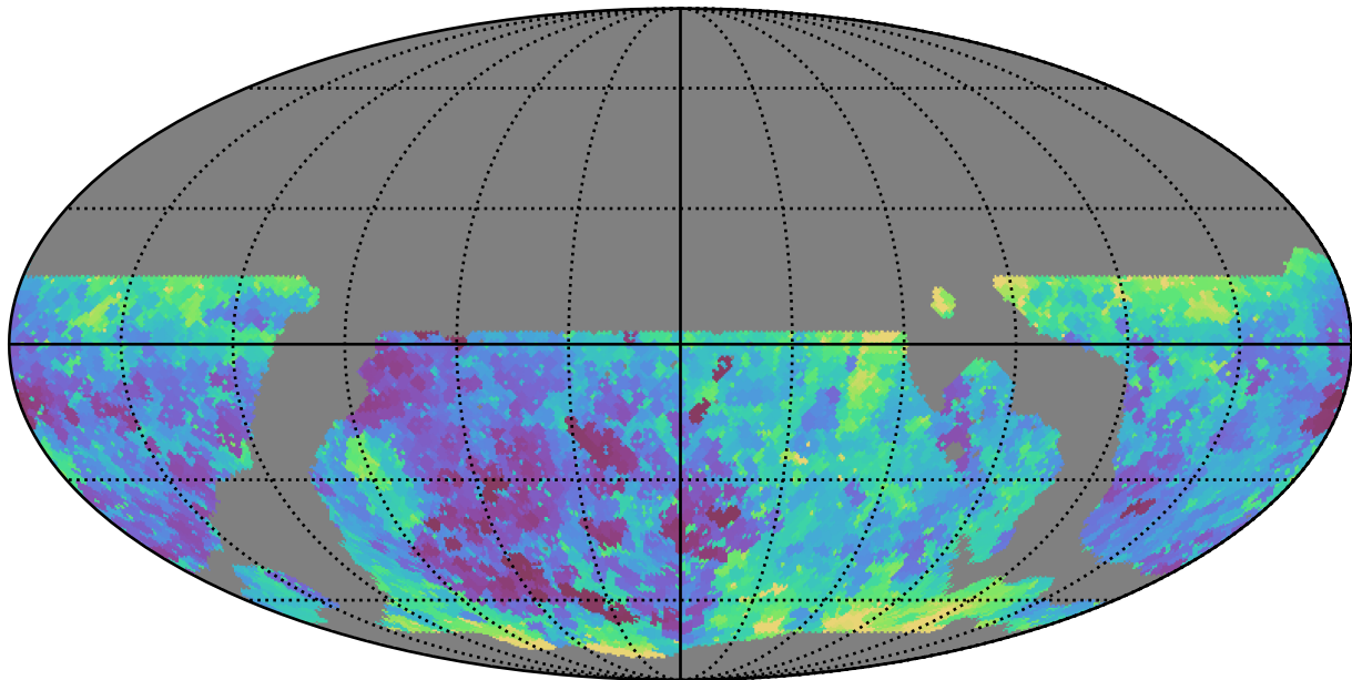
ddf_loaded_half_fl1_v3.4_10yrs WFD g band: Min seeingEff
