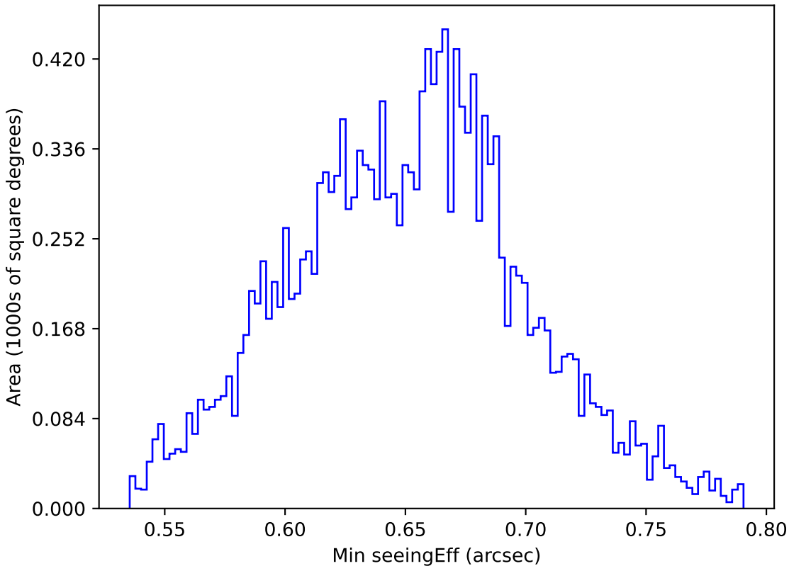
ddf_loaded_half_fl1_v3.4_10yrs WFD g band: Min seeingEff
