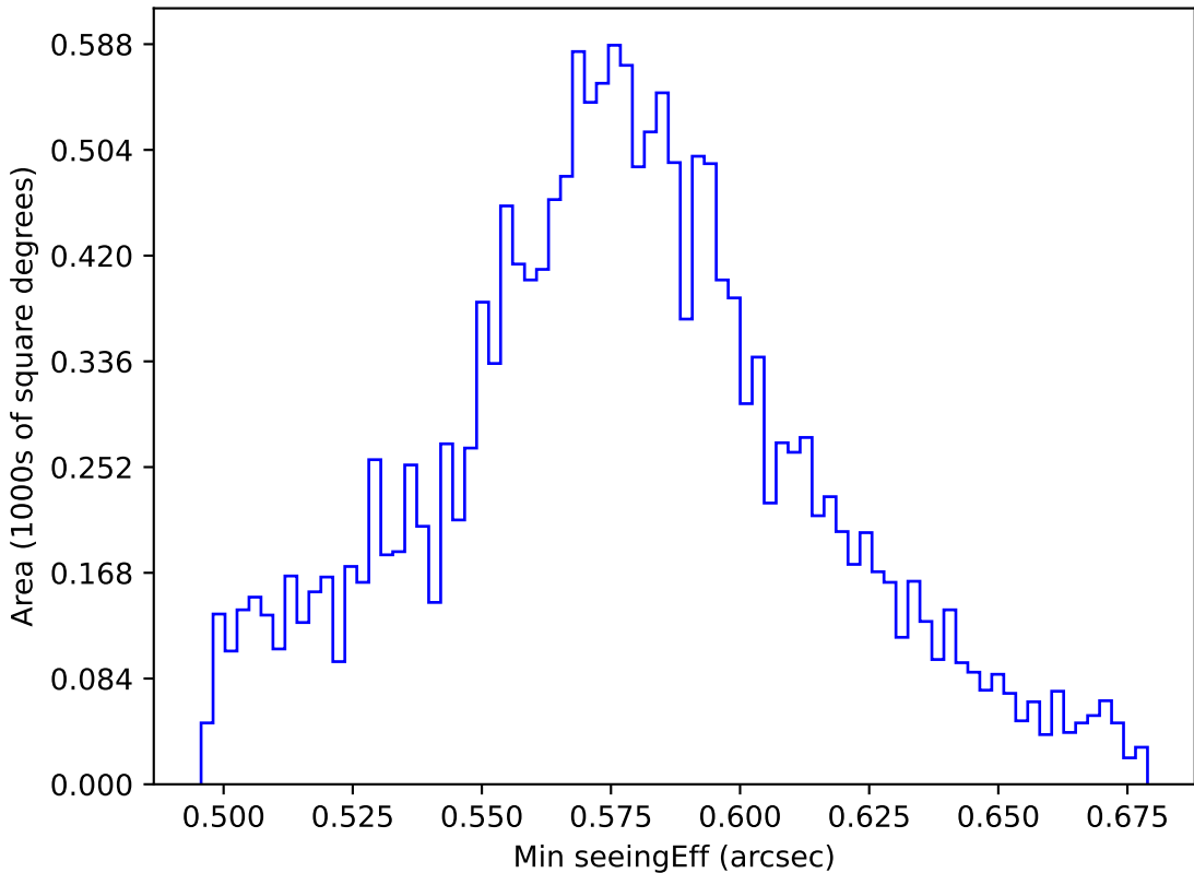
ddf_loaded_half_fl1_v3.4_10yrs WFD all bands: Min seeingEff
