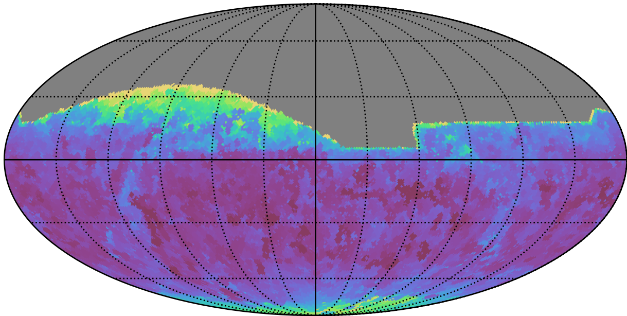
ddf_loaded_half_fl1_v3.4_10yrs All sky z band: Min seeingEff
