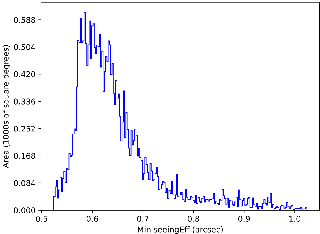
ddf_loaded_half_fl1_v3.4_10yrs All sky z band: Min seeingEff
