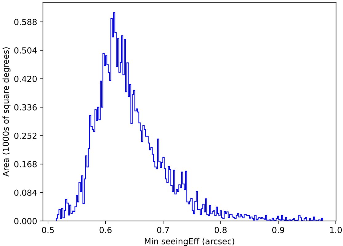
ddf_loaded_half_fl1_v3.4_10yrs All sky y band: Min seeingEff
