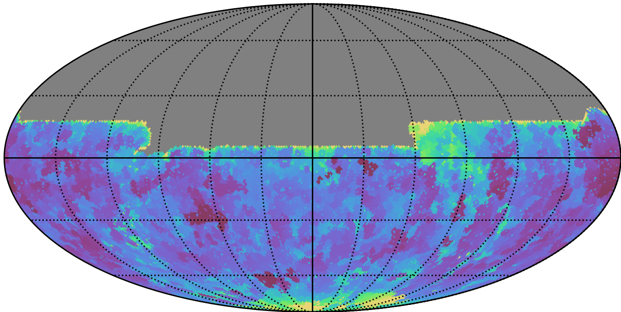
ddf_loaded_half_fl1_v3.4_10yrs All sky u band: Min seeingEff
