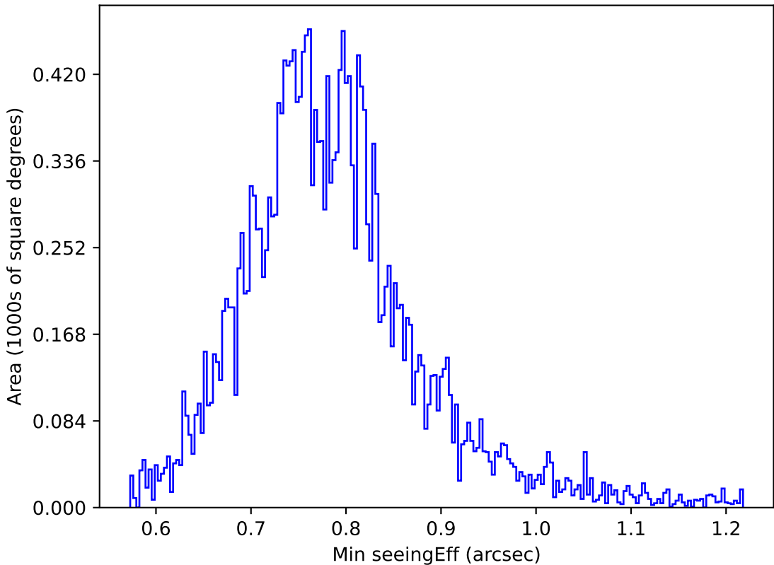
ddf_loaded_half_fl1_v3.4_10yrs All sky u band: Min seeingEff
