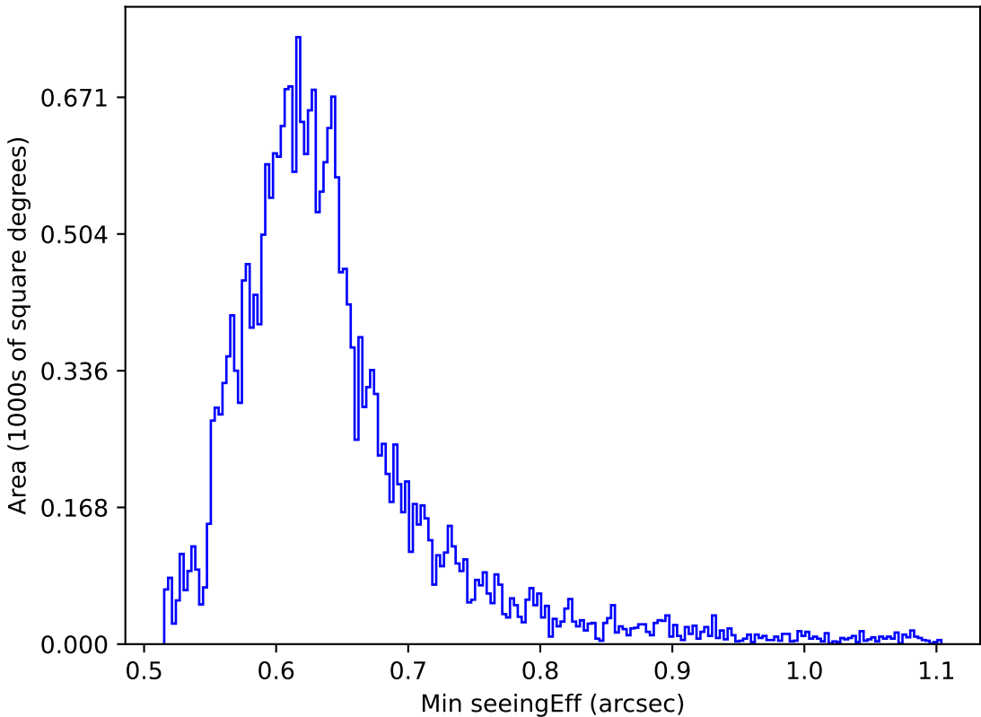
ddf_loaded_half_fl1_v3.4_10yrs All sky r band: Min seeingEff
