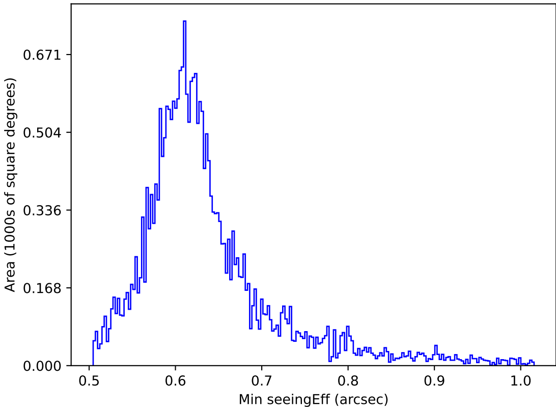
ddf_loaded_half_fl1_v3.4_10yrs All sky i band: Min seeingEff
