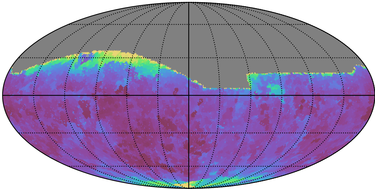
ddf_loaded_half_fl1_v3.4_10yrs All sky g band: Min seeingEff
