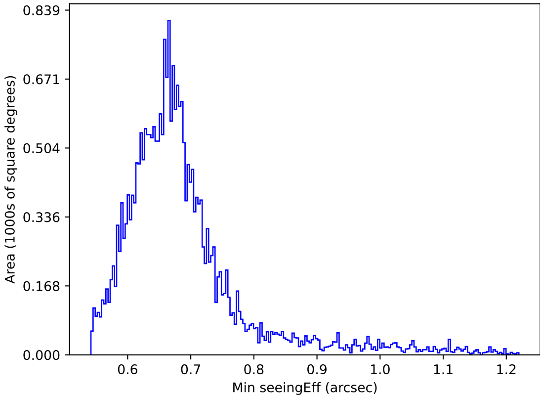
ddf_loaded_half_fl1_v3.4_10yrs All sky g band: Min seeingEff
