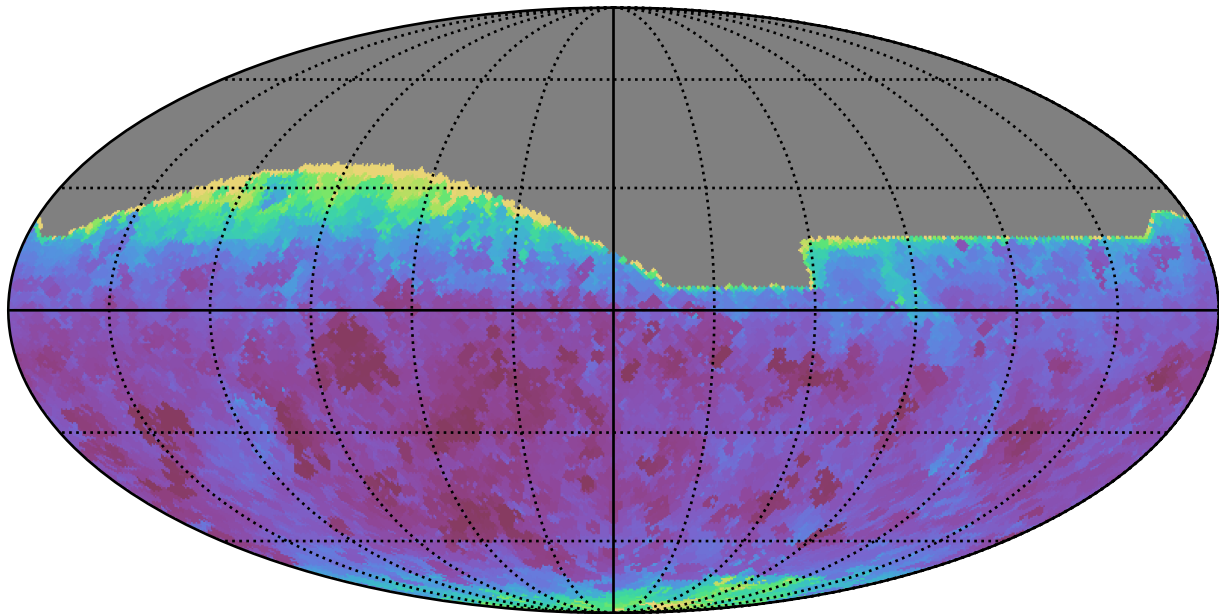
ddf_loaded_half_fl1_v3.4_10yrs All sky all bands: Min seeingEff
