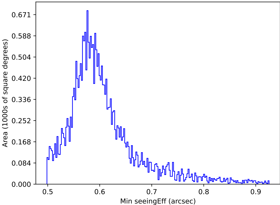
ddf_loaded_half_fl1_v3.4_10yrs All sky all bands: Min seeingEff
