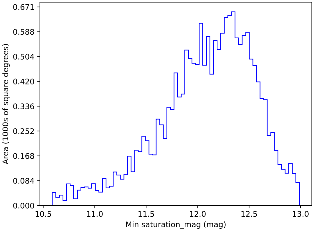
ddf_loaded_half_fl1_v3.4_10yrs WFD z band: Min saturation_mag
